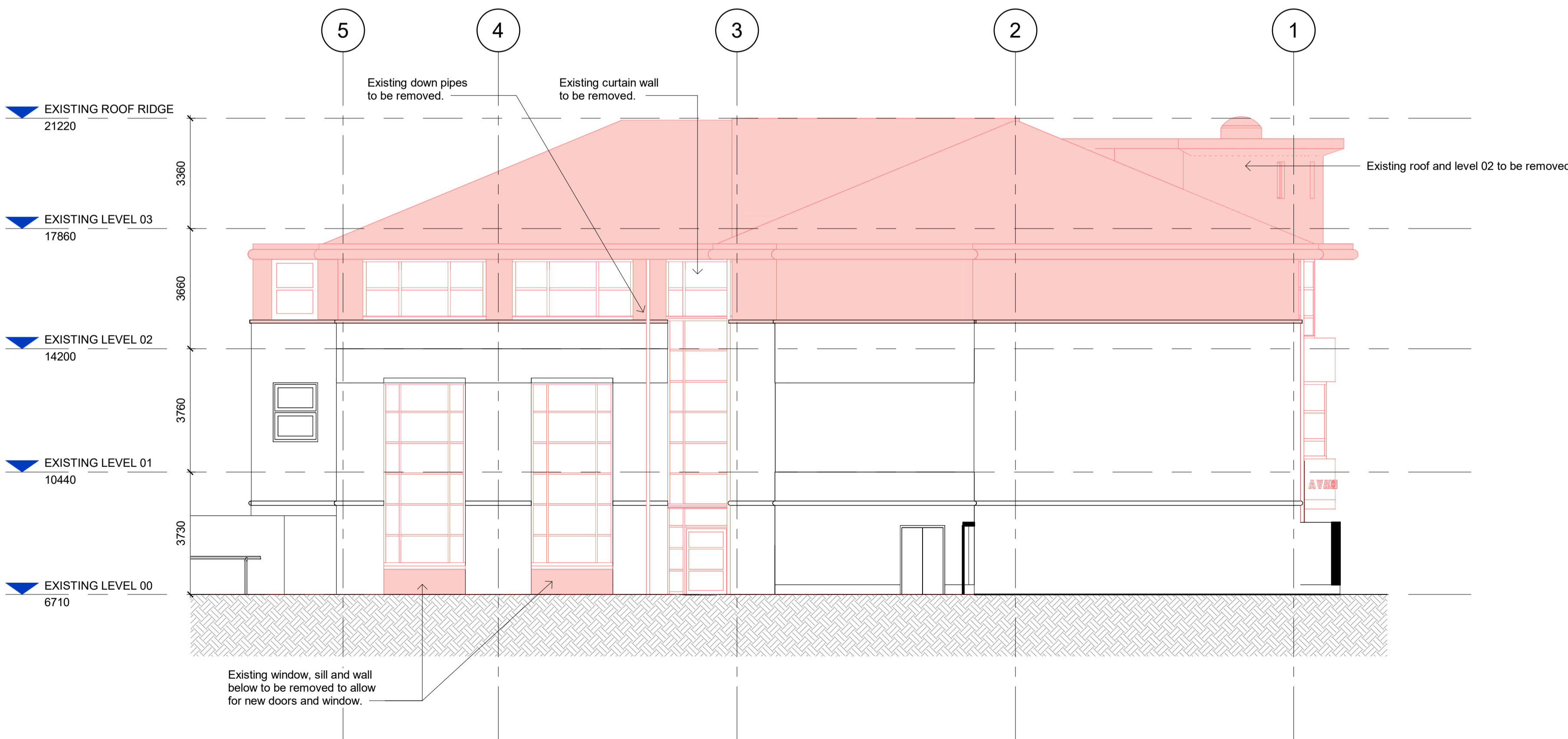
2 Demolition Elevation - East 1 : 100
