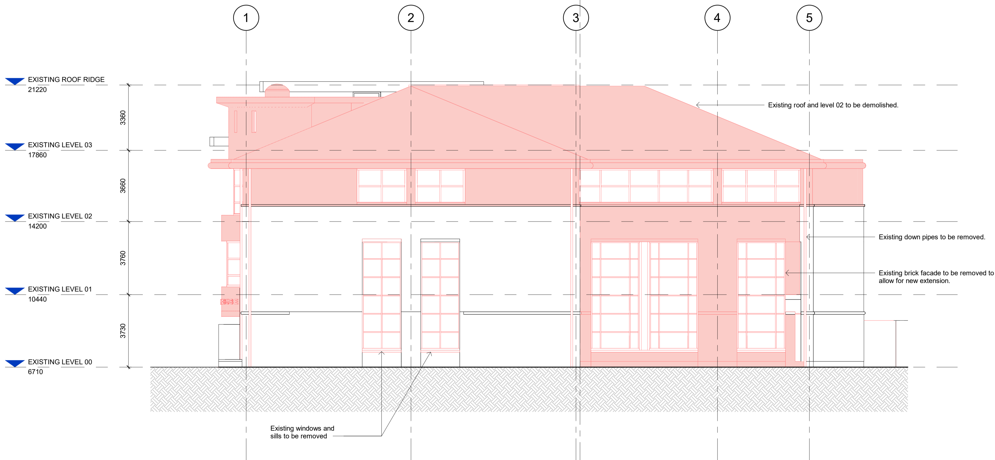
2 Demolition Elevation - West 1 : 100
