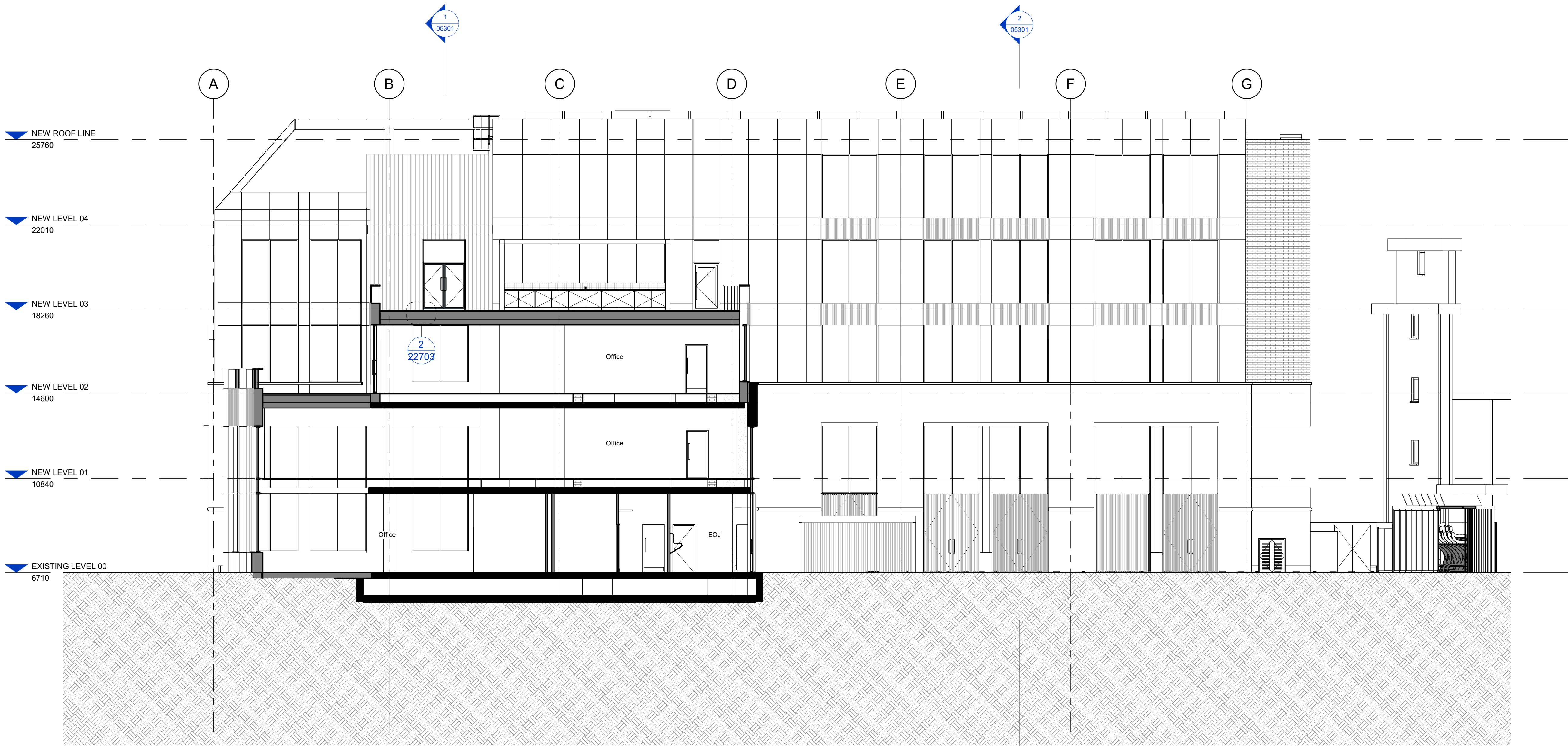
1 Proposed Section D-D 1 : 100
