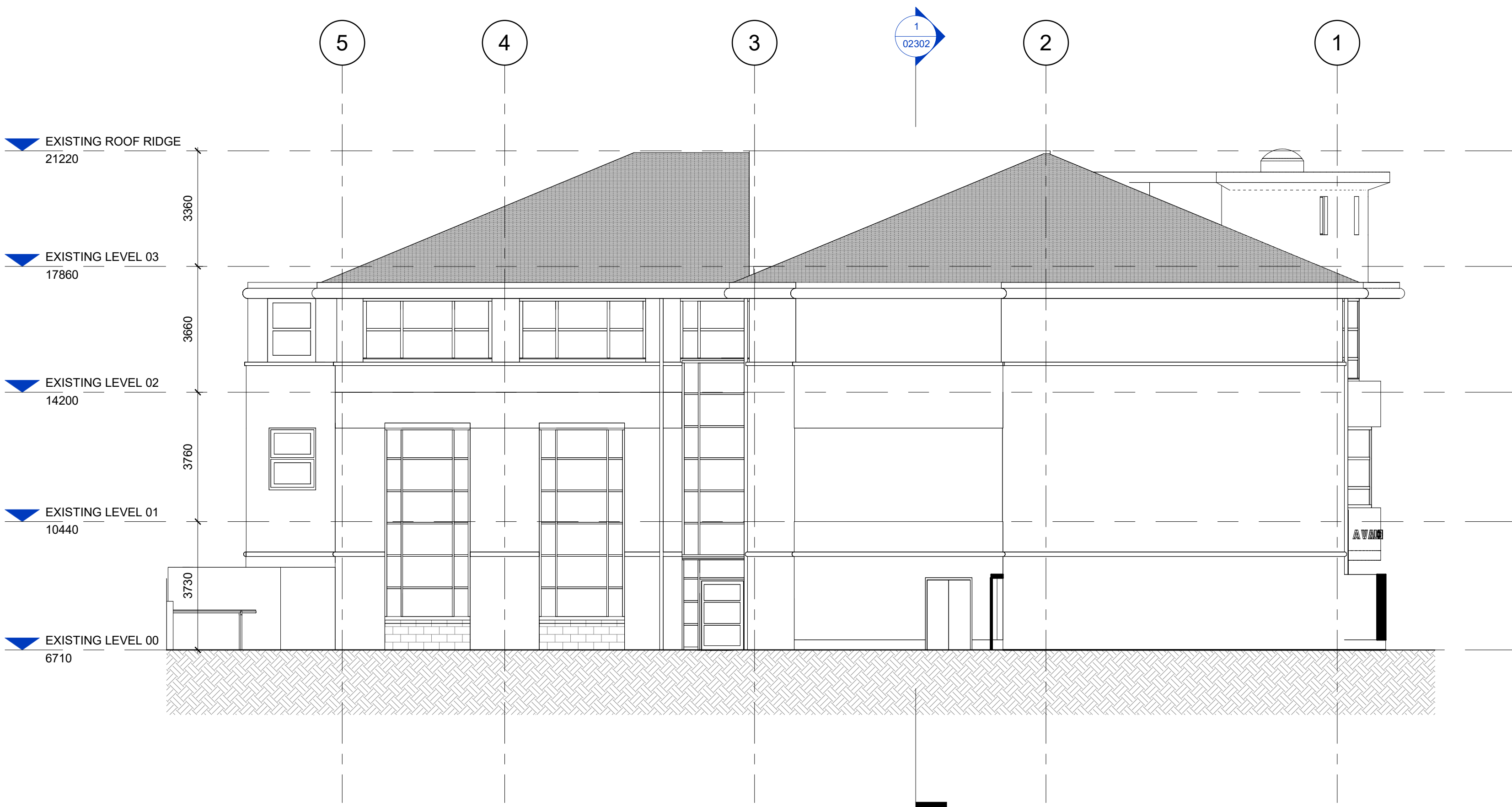
2 Existing Elevation - East 1 : 100
