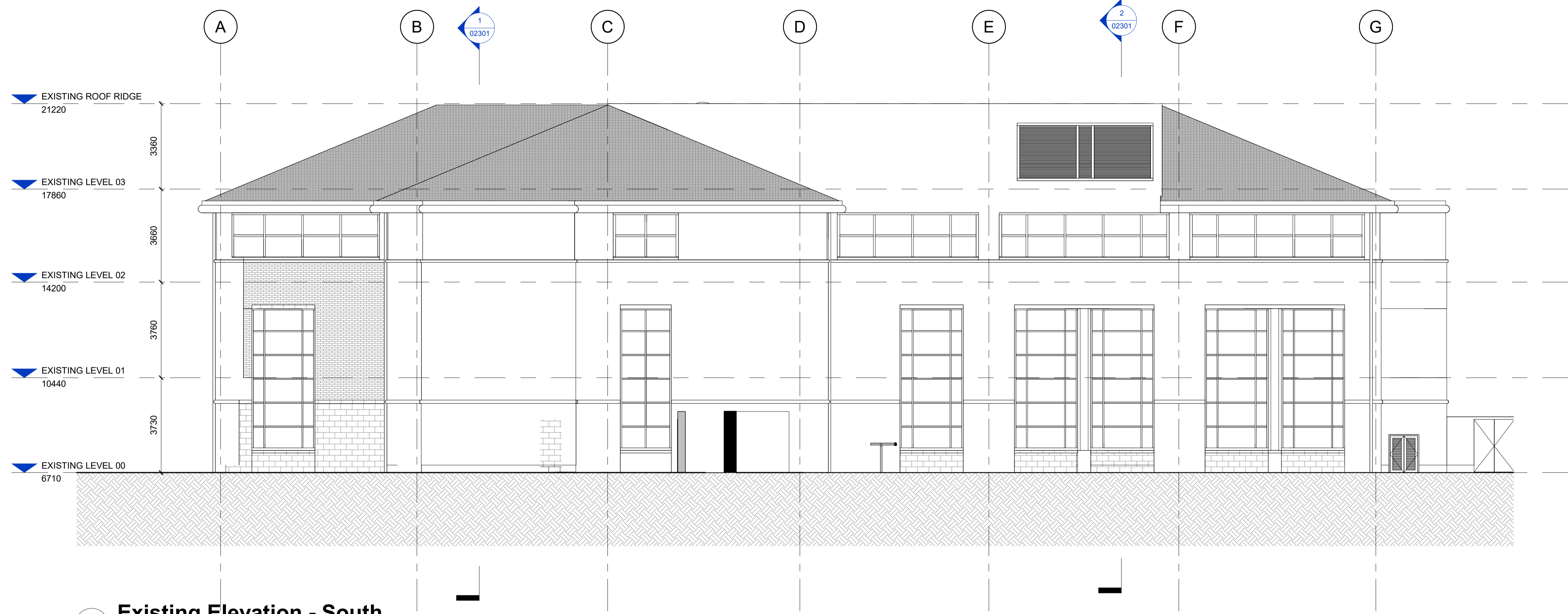
1 Existing Elevation - South 1 : 100
