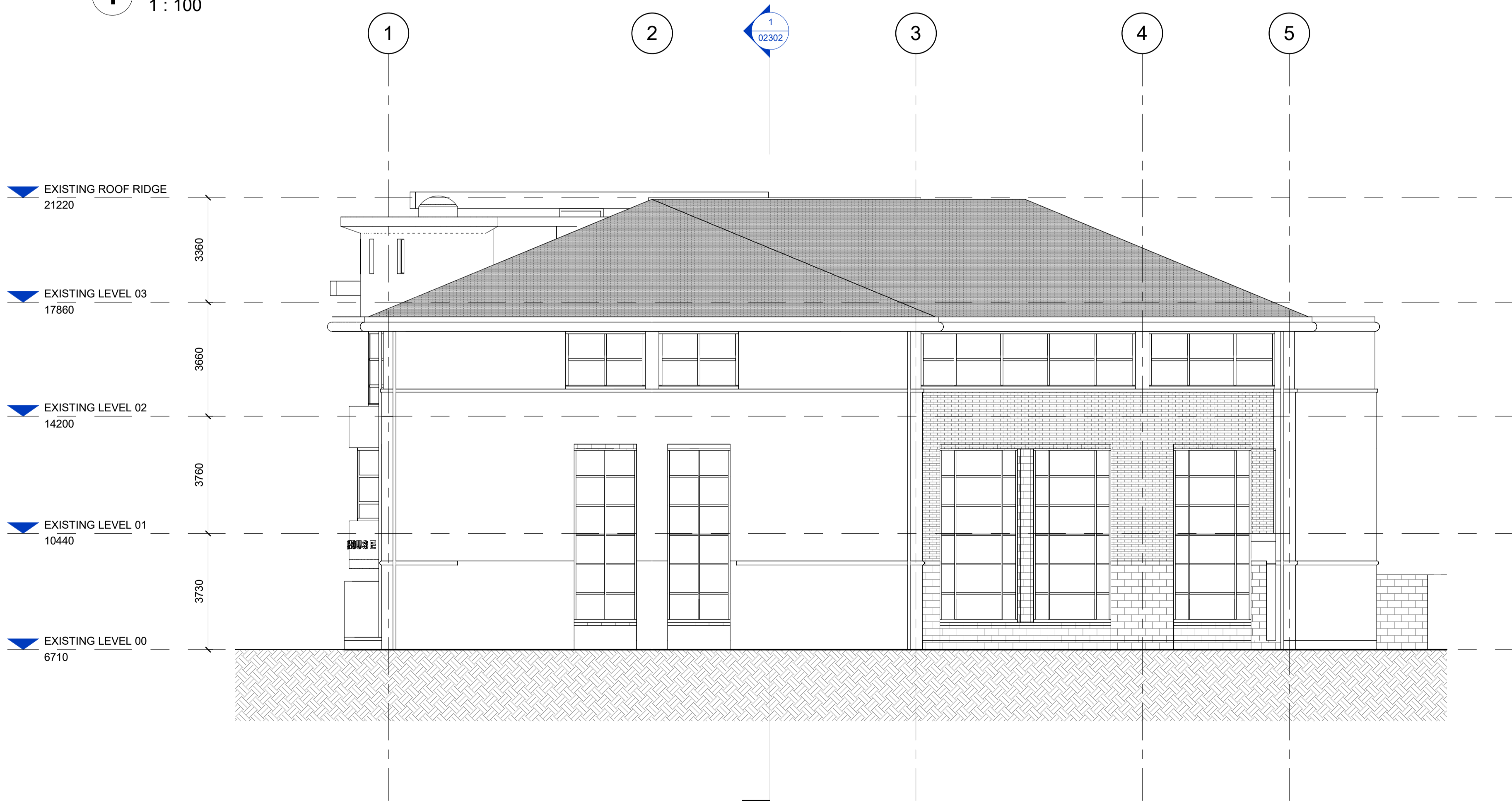
2 Existing Elevation - West 1 : 100
