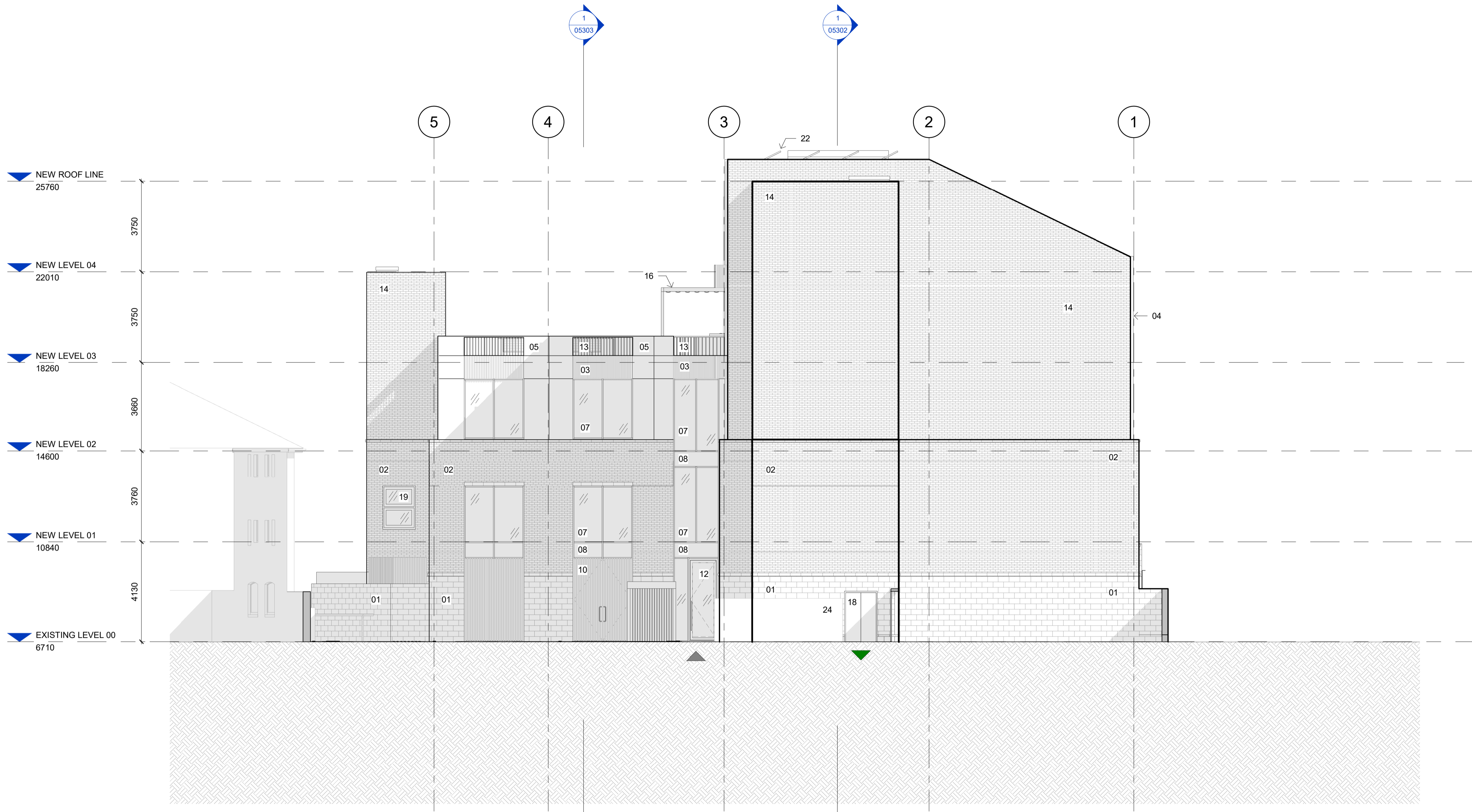
1 Proposed Elevation - East 1 : 100
