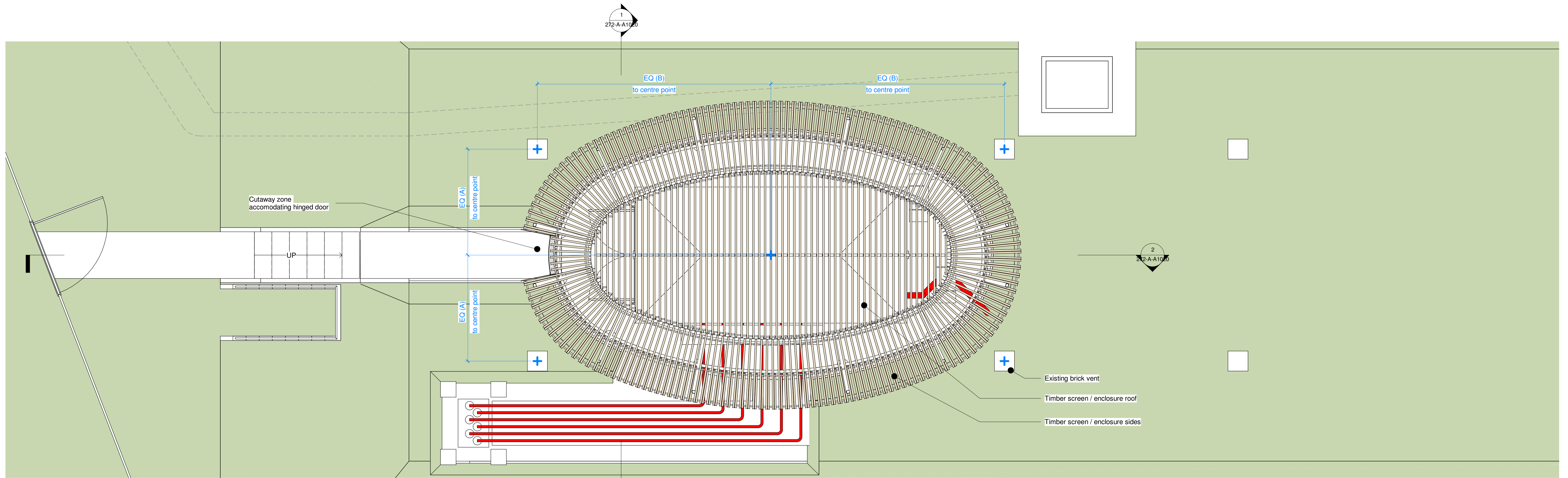
1 Roof Level 1 : 50
