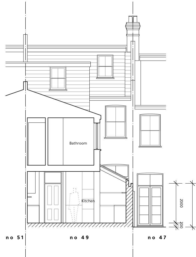
SECTION BB
