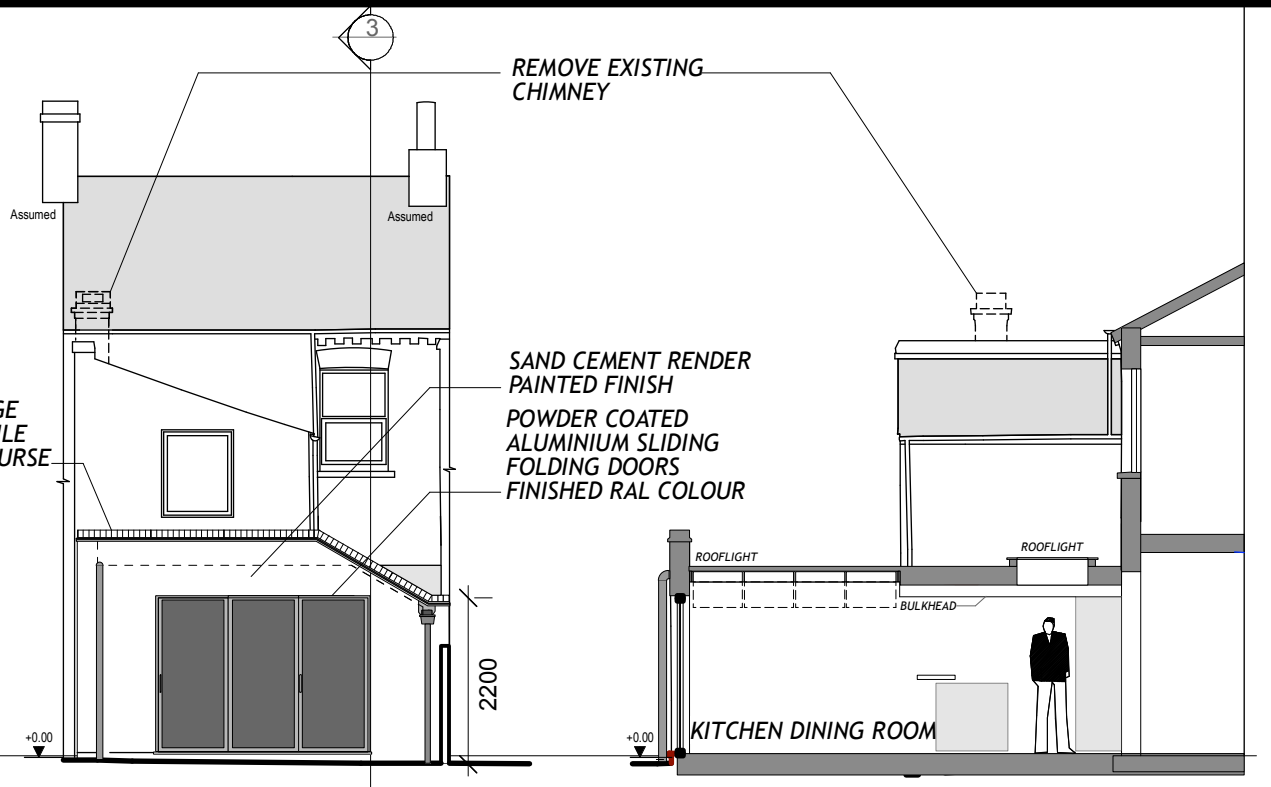
REAR ELEVATION PROPOSED
