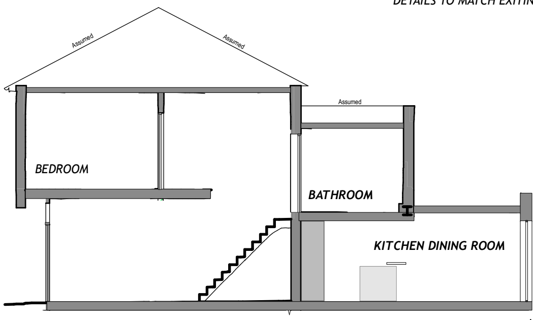
SECTION 1 PROPOSED
