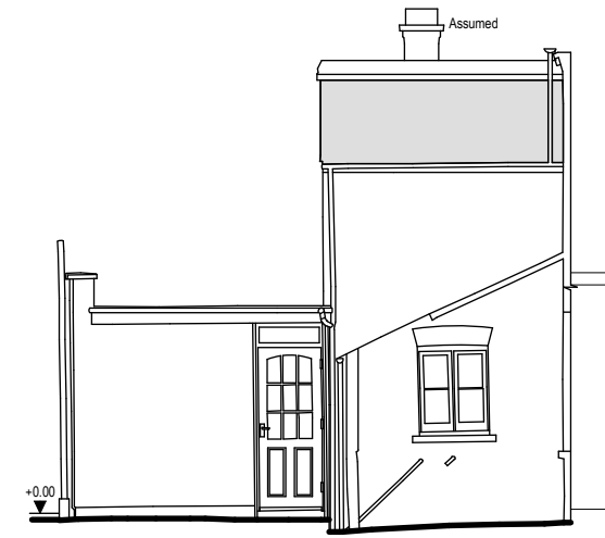
SIDE ELEVATION EXISTING
