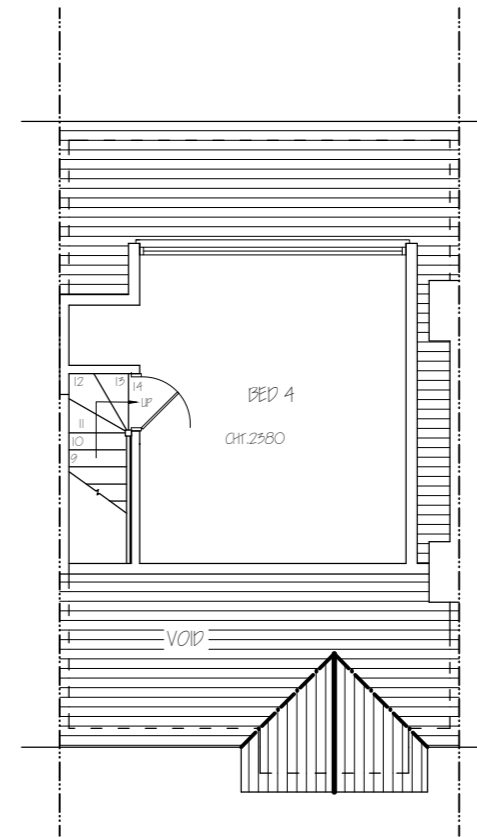
EXISTING LOFT FLOOR PLAN
