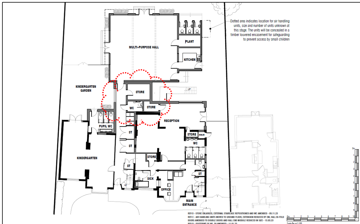
Figure 1 - Proposed ground floor plan showing revised link section
