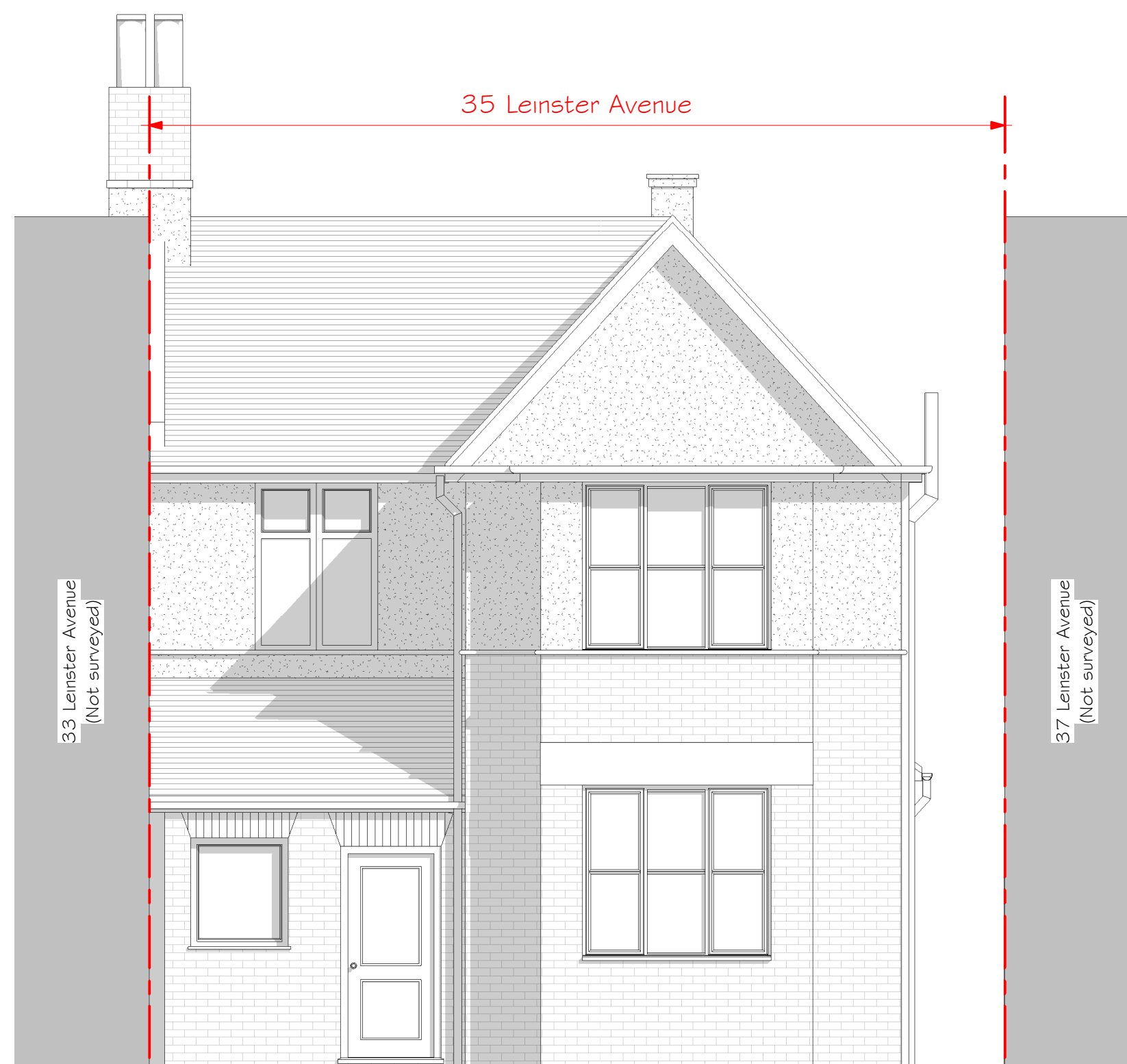
1 Existing Front(North) Elevation 1 : 50
