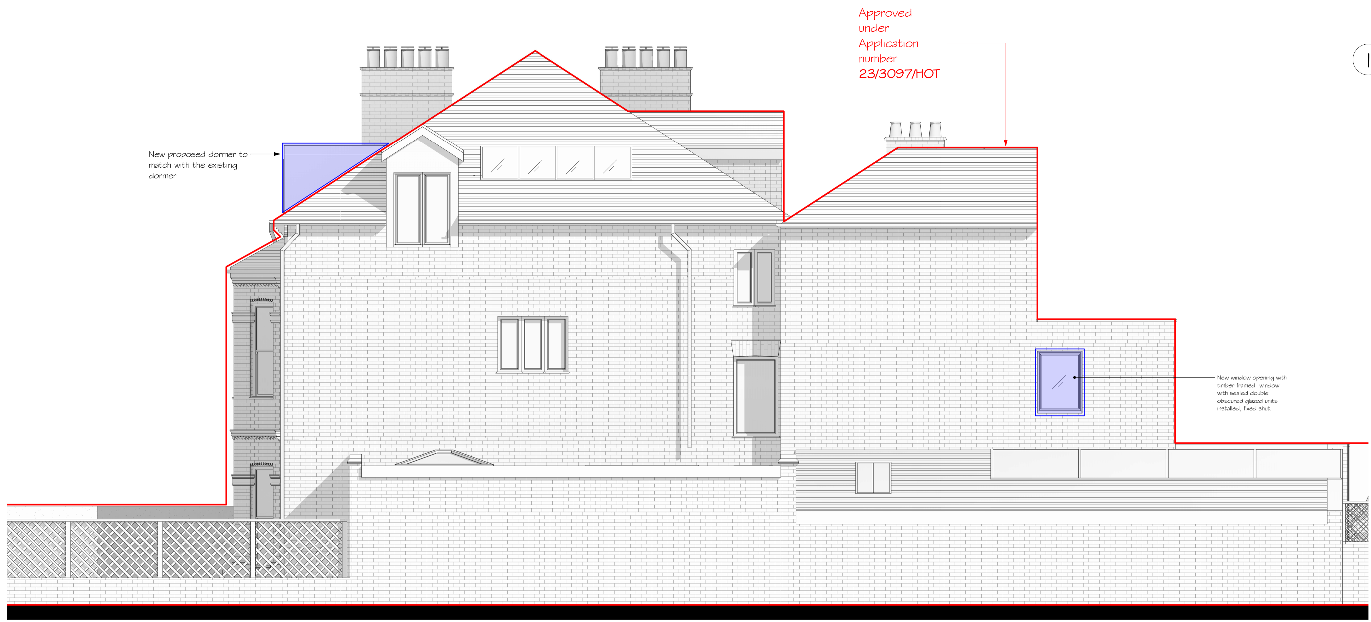
4 Proposed North Elevation 1 : 50
