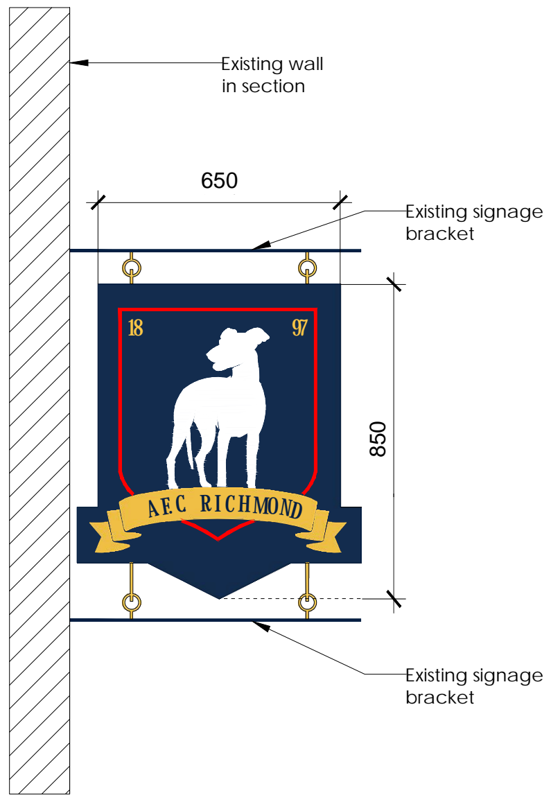
Signage detail Scale 1:20@A3
