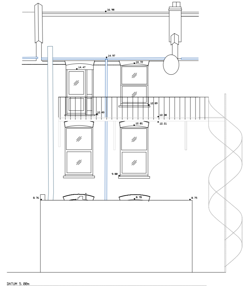
REAR ELEVATION
