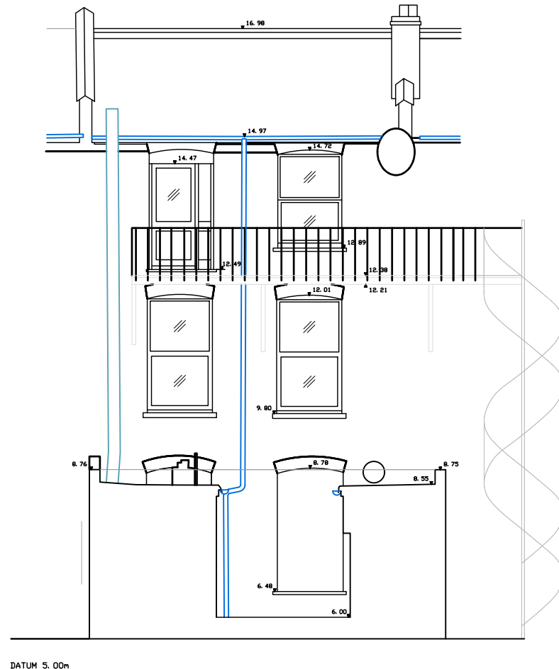
DATUM 5.00m REAR ELEVATION (THRU LIGHTWELL)
