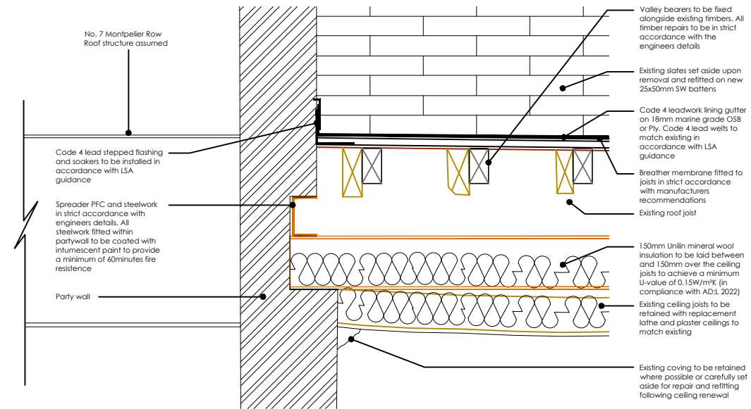
DETAIL A - PARTY WALL/VALLEY DETAIL
