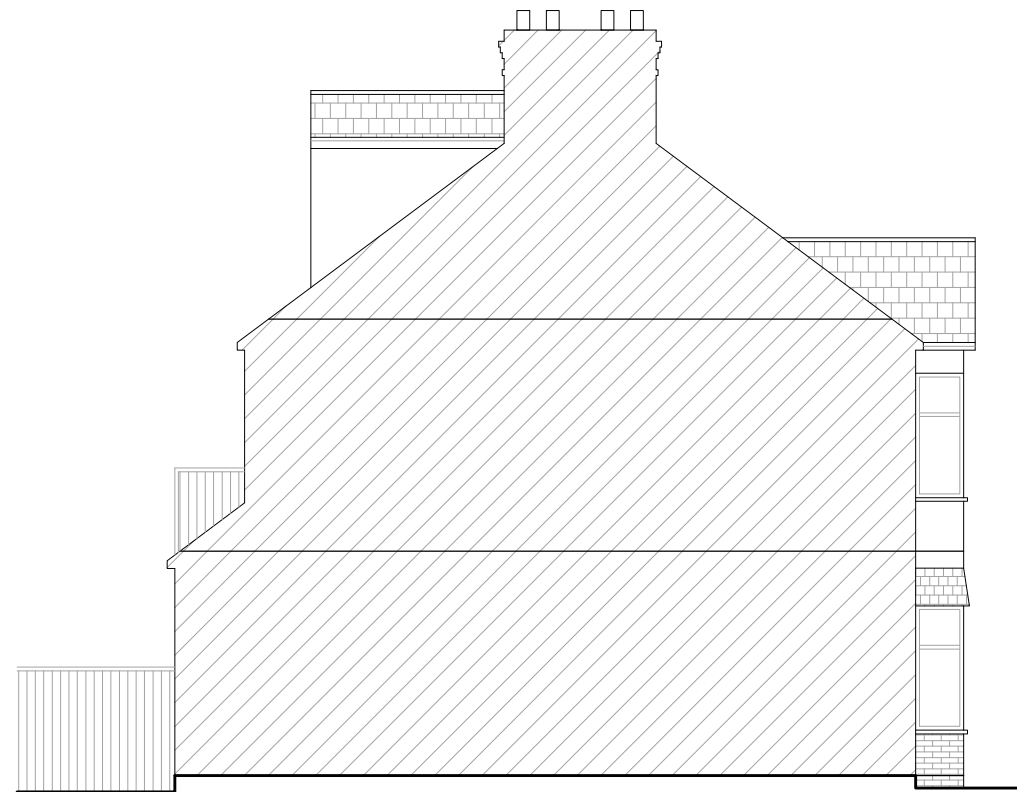
02 Existing Side Elevation 1:100 @ A3
