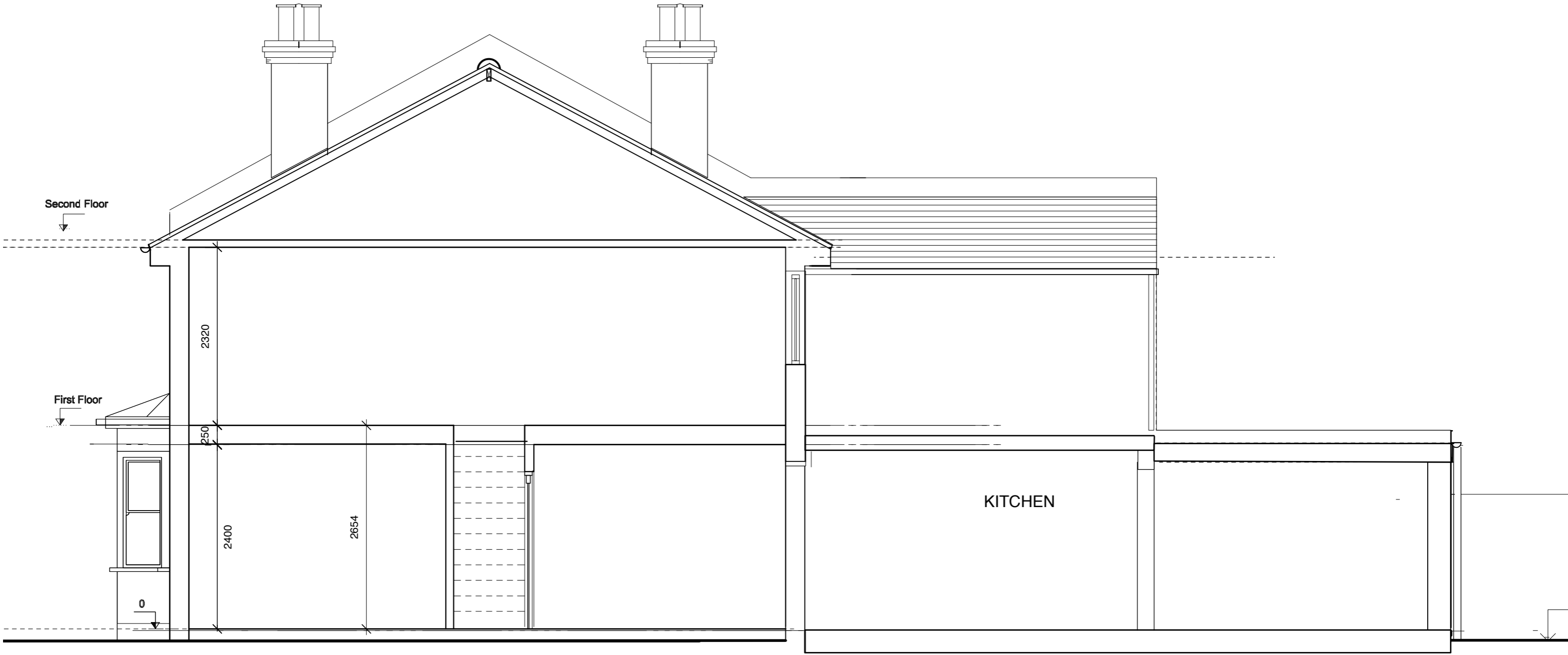
PROPOSED SECTION 1:50
