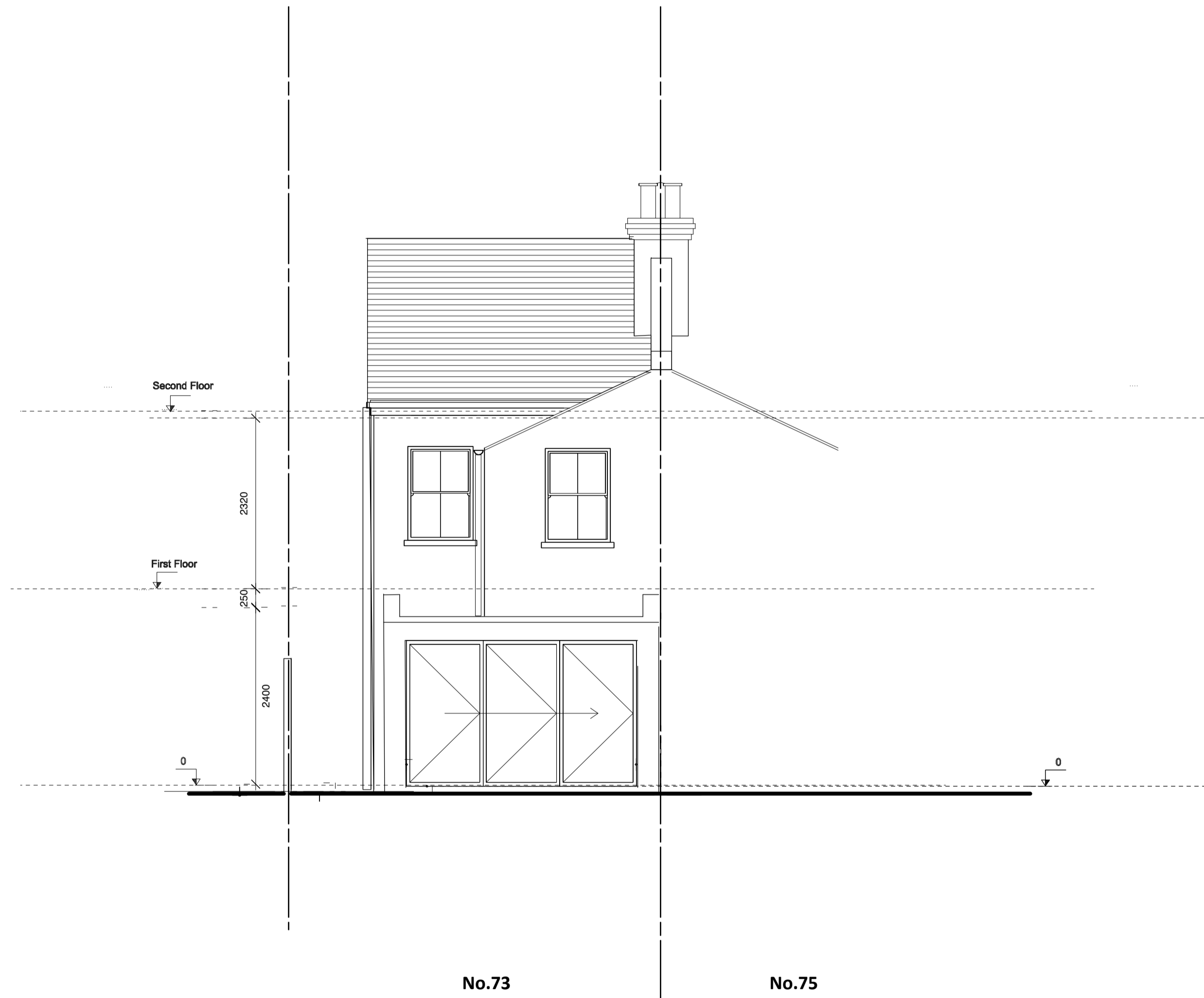
EXISTING REAR ELEVATION 1:50
