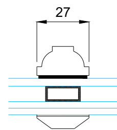
Glazing bar detail
