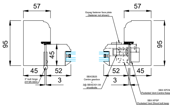
Horizontal section
