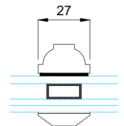
Glazing bar detail
