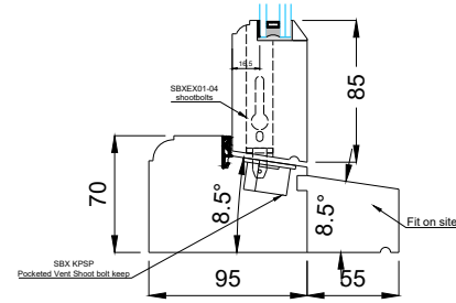
Vertical section
