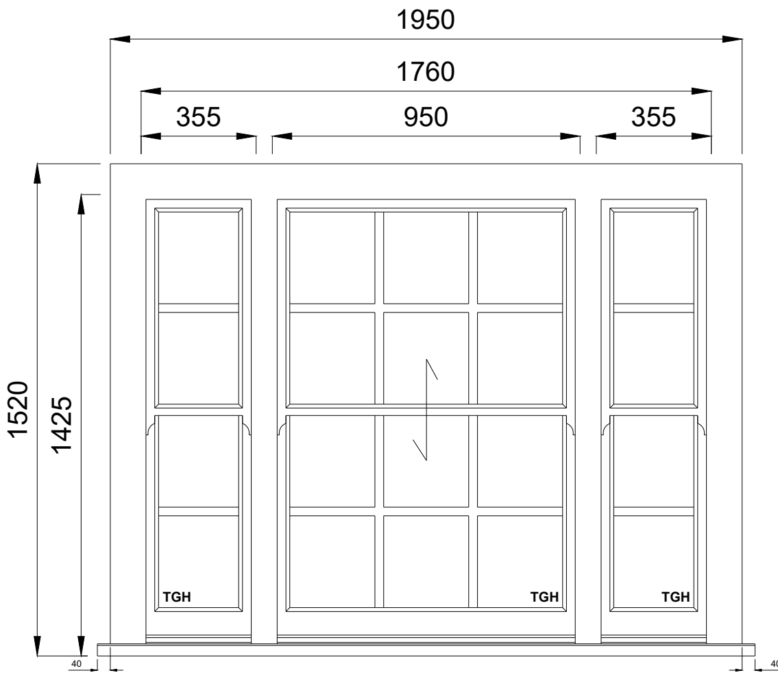
W4 1st fl - Rear Elev. Master Bedroom Qty 1 Viewed from outside
