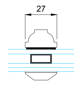
Glazing bar detail
