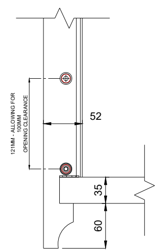
Horn & opening restrictor detail
