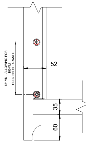
Horn & opening restrictor detail
