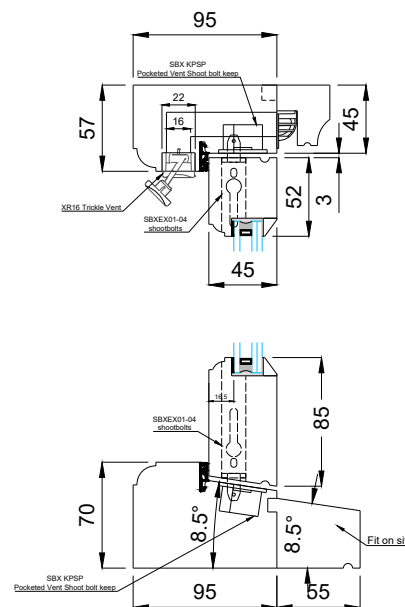
Vertical section
