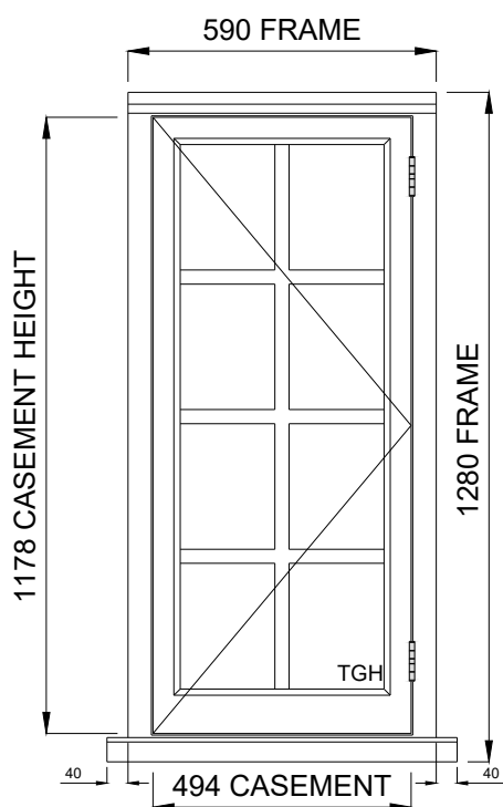
W7 1st fl - Front Elev. WC Landing Qty 1 Viewed from outside Open outwards
