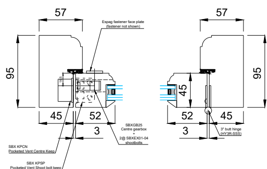
Horizontal section
