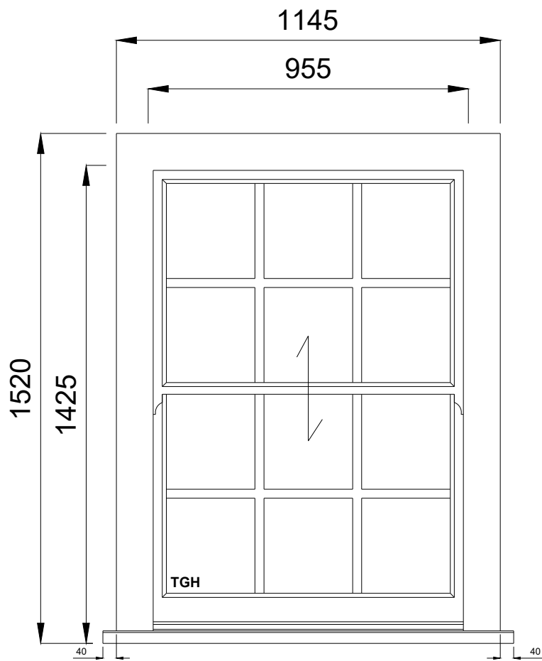
W9 Gfl - Front Elev. Kitchen Qty 1 Viewed from outside
