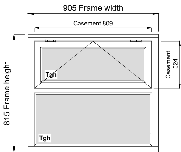
W.10 GFL - Side Elev. - Boiler Room Qty 1 Viewed from outside Open outwards
