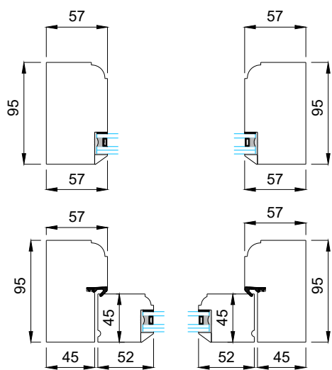
Horizontal section
