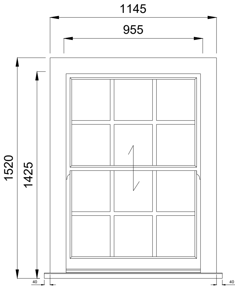
W12 Gfl - Front Elev. Lounge Qty 1 Viewed from outside
