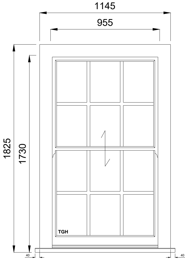
W13 Gfl - Rear Elev. Lounge Qty 1 Viewed from outside
