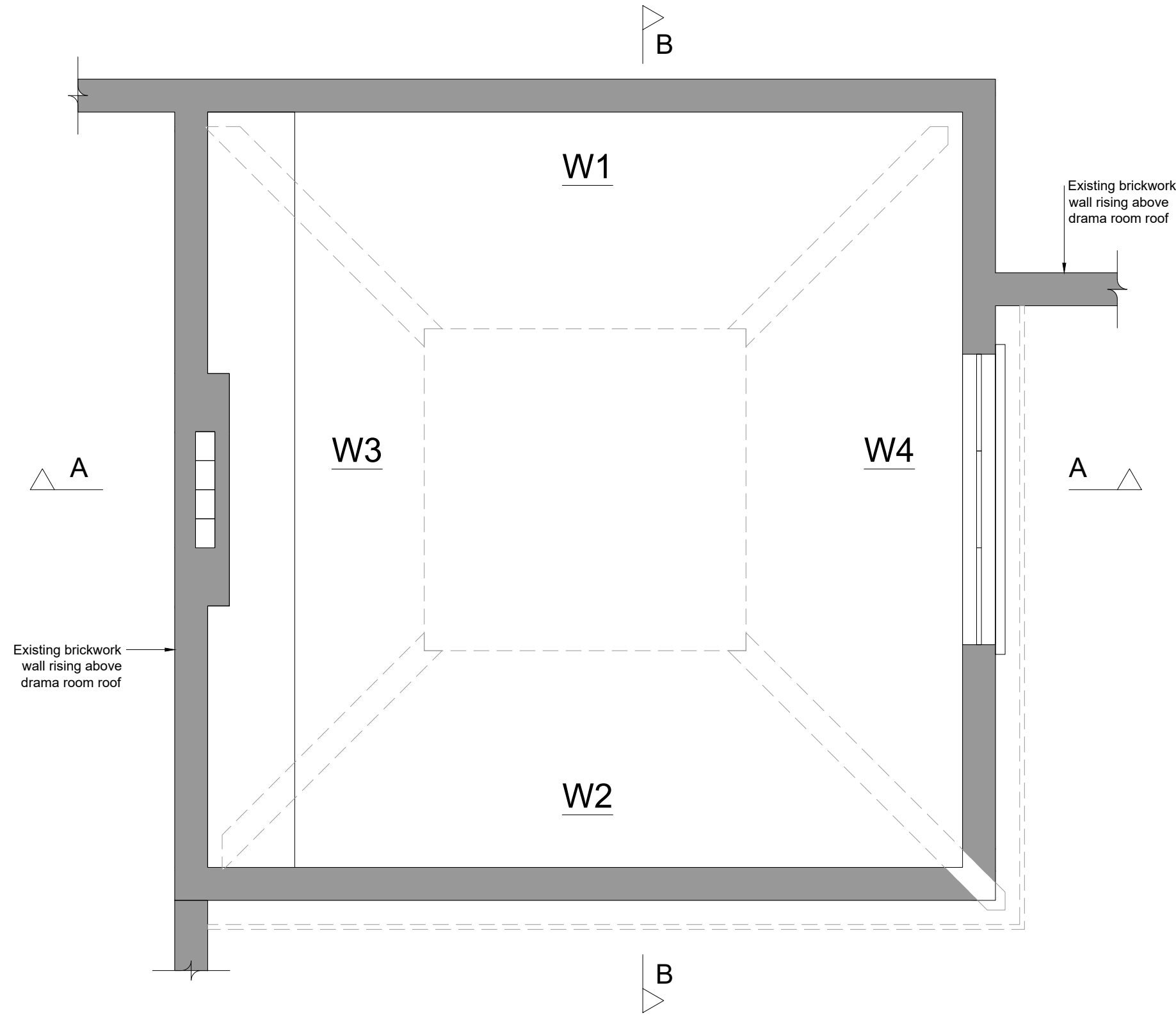
Drama Room Existing and Proposed Floor Plan
