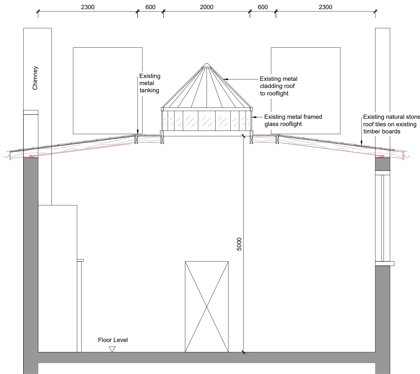
Drama Room Section A-A - full height Wall W1
