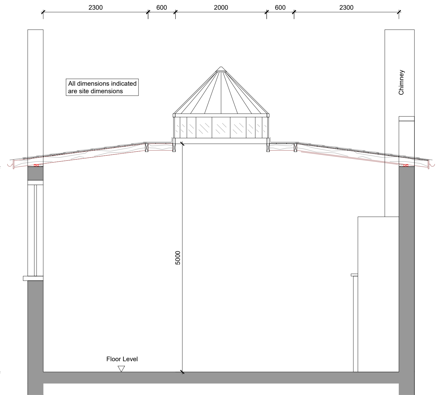
Drama Room Section A-A - full height - handed Wall W2
