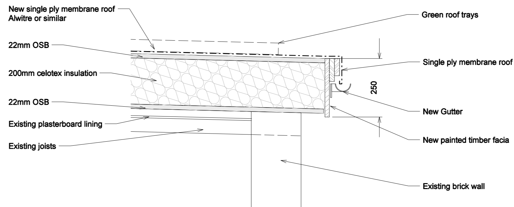
Typical eaves detail
