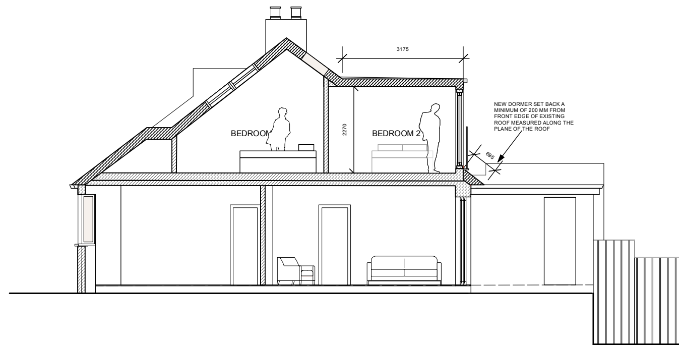
PROPOSED SECTION DD
