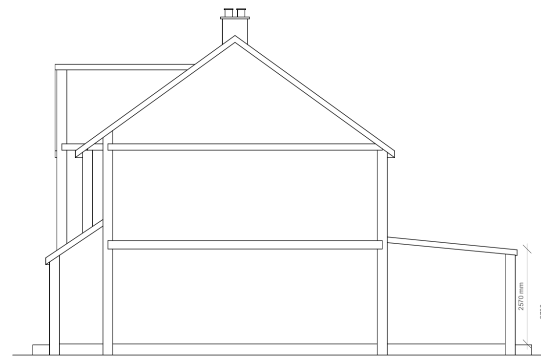
EXISTING RIGHT SIDE SECTION
