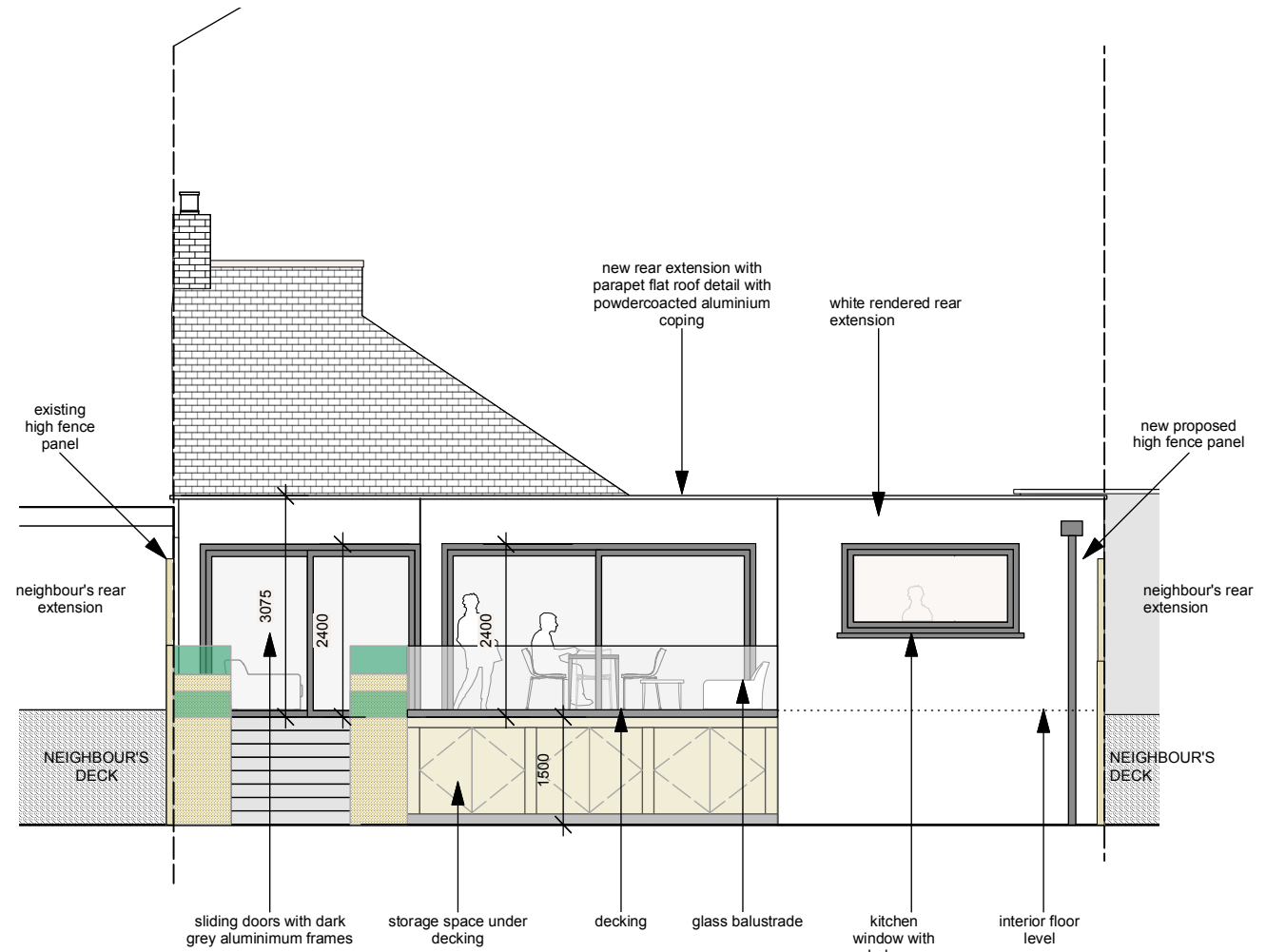
PROPOSED REAR ELEVATION BB
