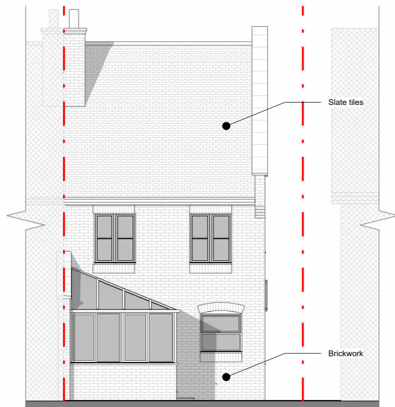
Rear Elevation
