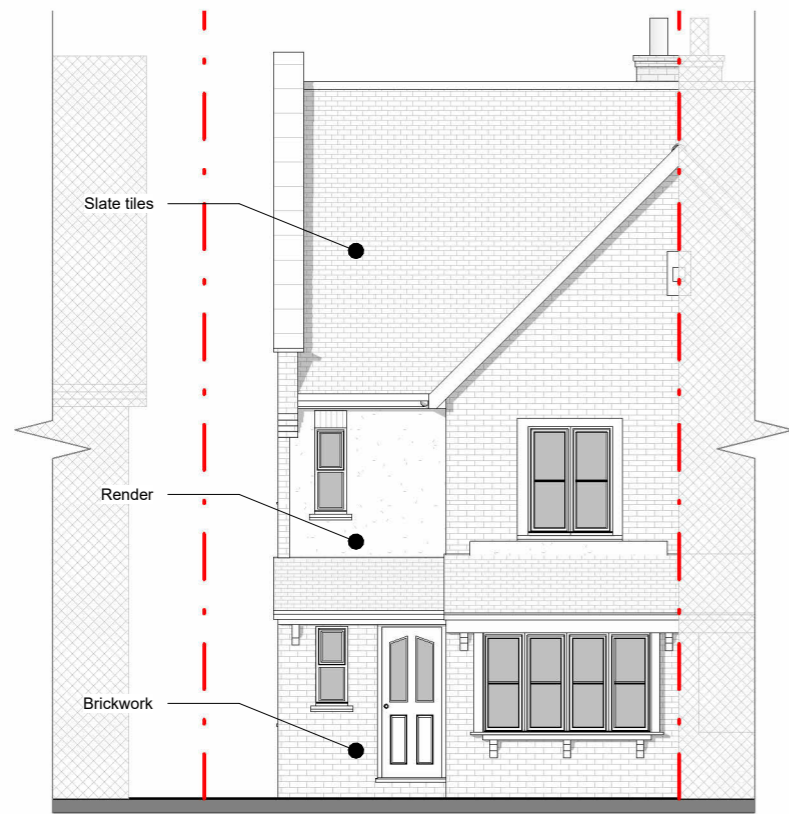
Front Elevation
