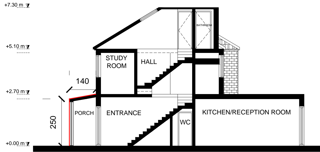
Proposed A-A Section
