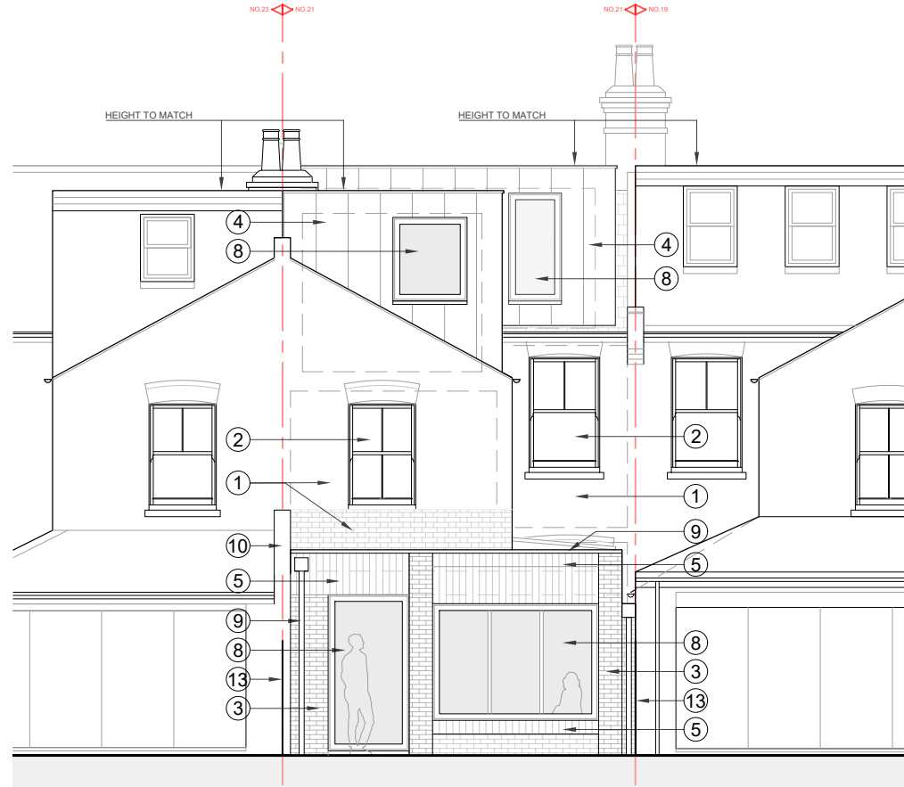
REAR ELEVATION - WEST (PROPOSED)
