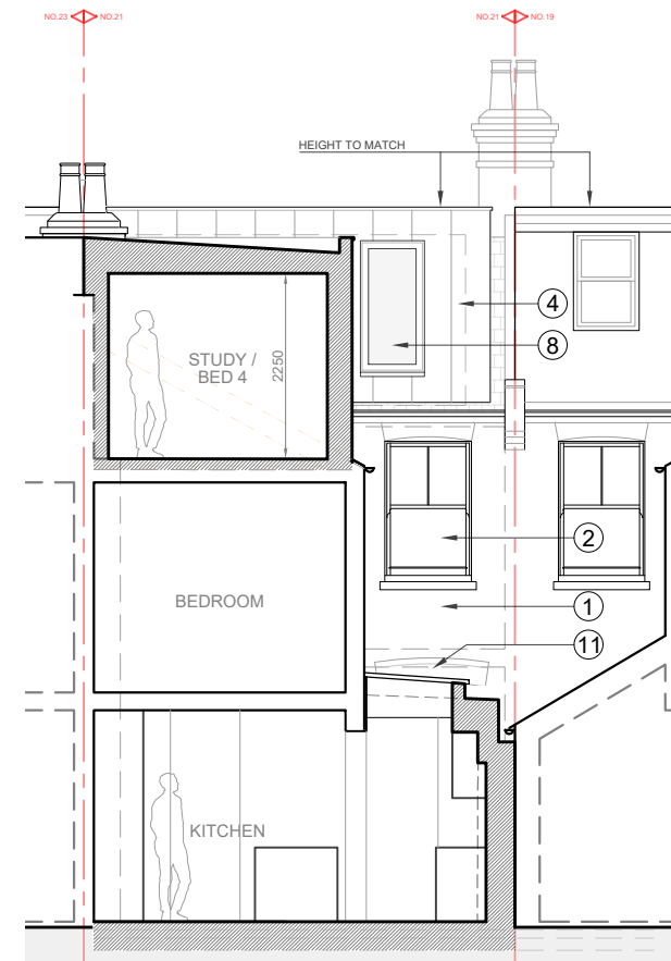
SECTION B-B (PROPOSED)
