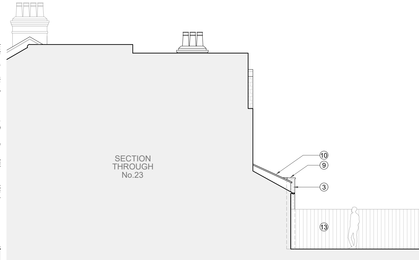
SIDE ELEVATION - NORTH (PROPOSED)
