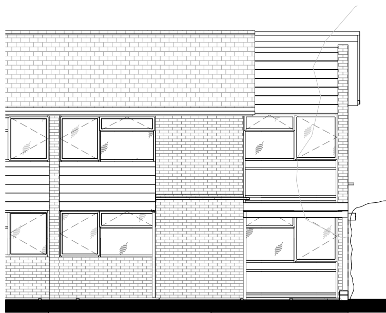
2 Elevation-East-Proposed
