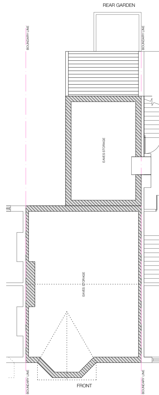
3 Existing Second Floor Plan 1:100 @ A3
