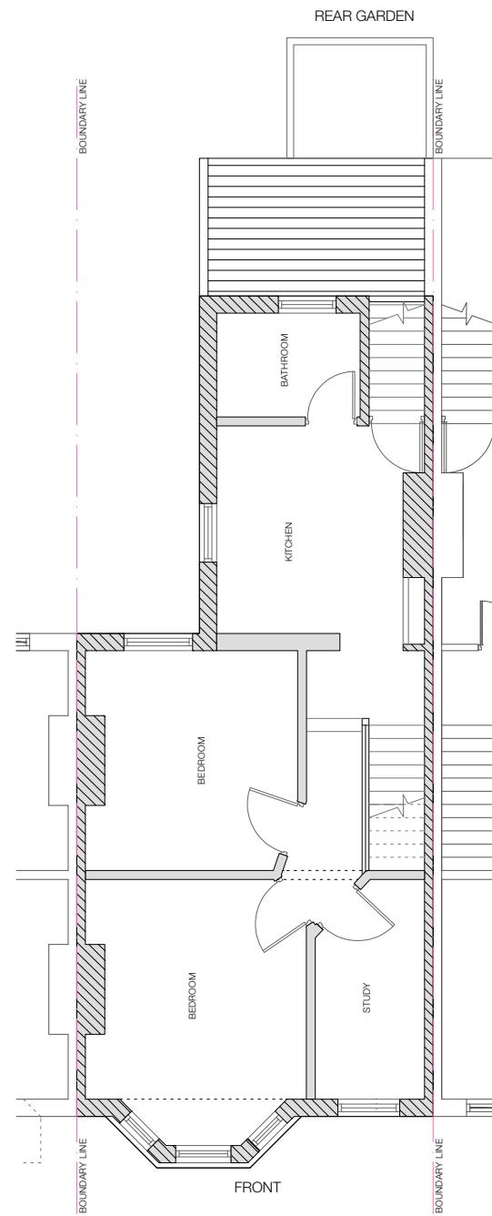
2 Existing First Floor Plan 1:100 @ A3
