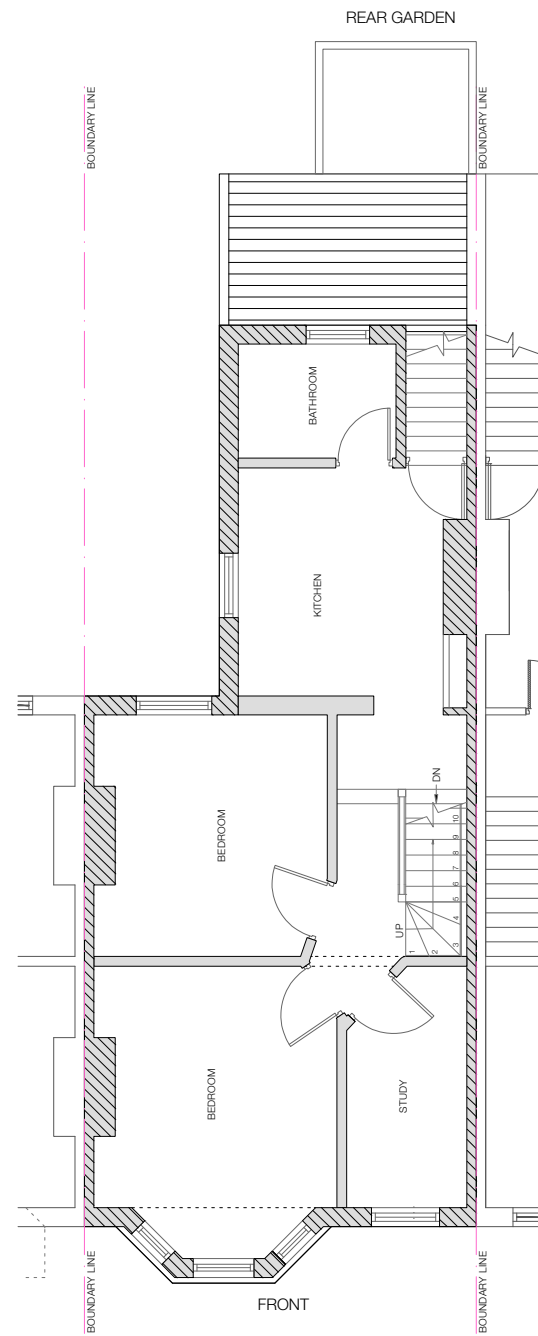
2 Proposed First Floor Plan 1:100 @ A3
