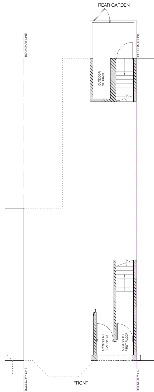
1 Proposed Ground Floor Plan 1:100 @ A3
