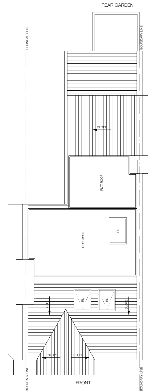
4 Proposed Roof Plan 1:100 @ A3
