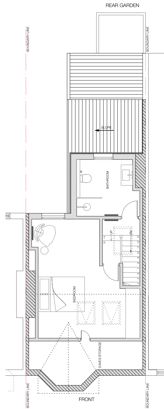
3 Proposed Second Floor Plan 1:100 @ A3
