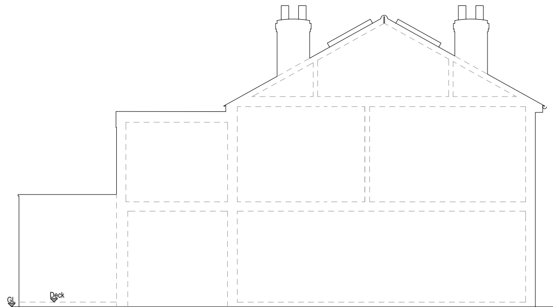
Side (N) Elevation Existing
