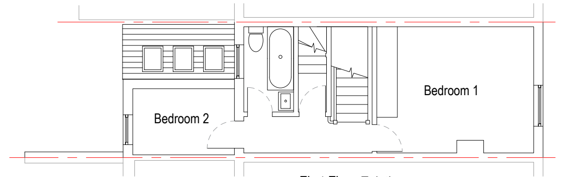
First Floor Existing
