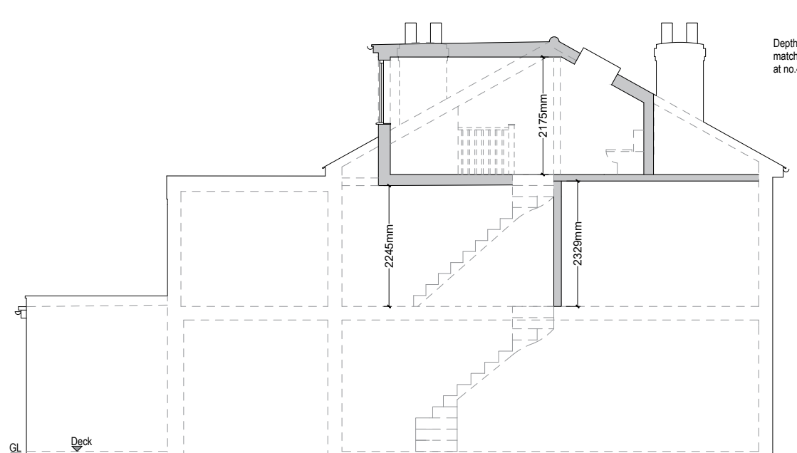
Side (N) Elevation Proposed
