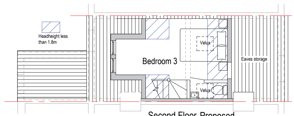
Second Floor Proposed
