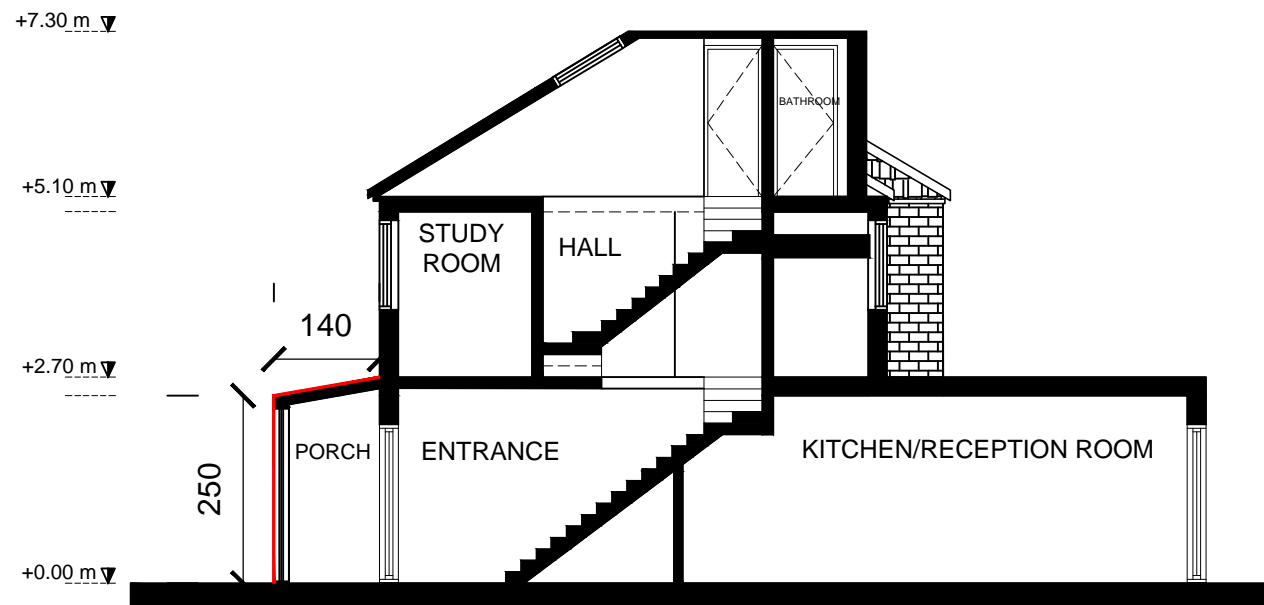
Proposed A-A Section
