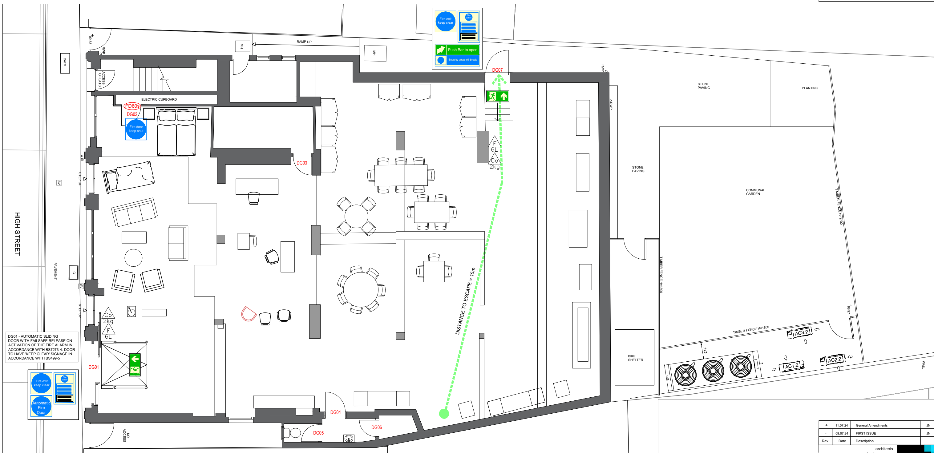
PROPOSED GROUND FLOOR FIRE STRATEGY (1:50@A1)
