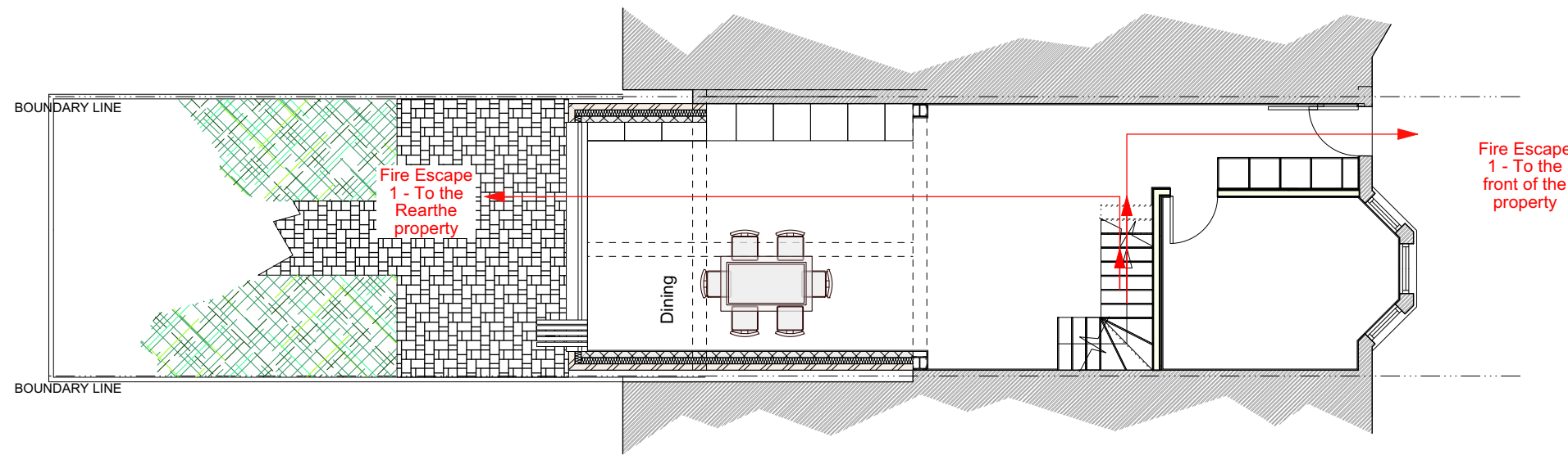
Fire Escape Routes
