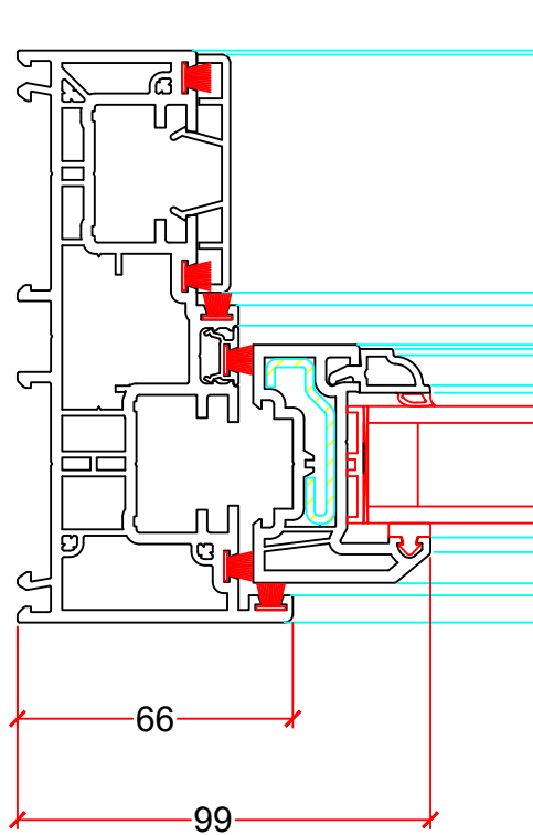
A-A Section Detail
