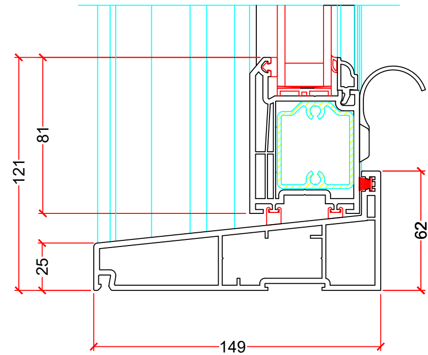
C-C Section Detail
