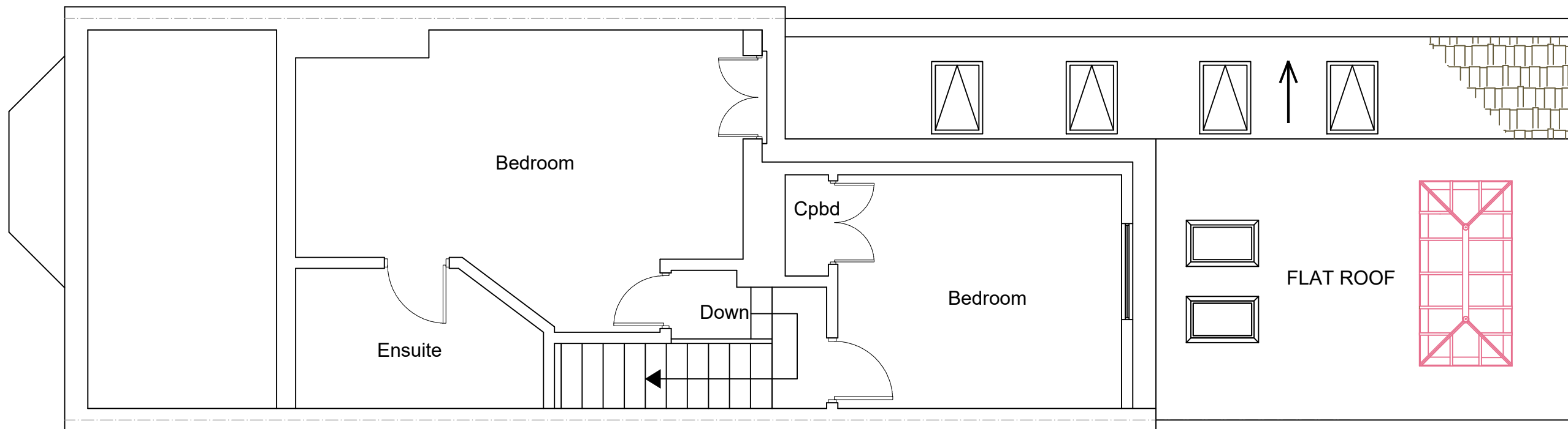
PROPOSED LOFT PLAN SCALE 1:50
