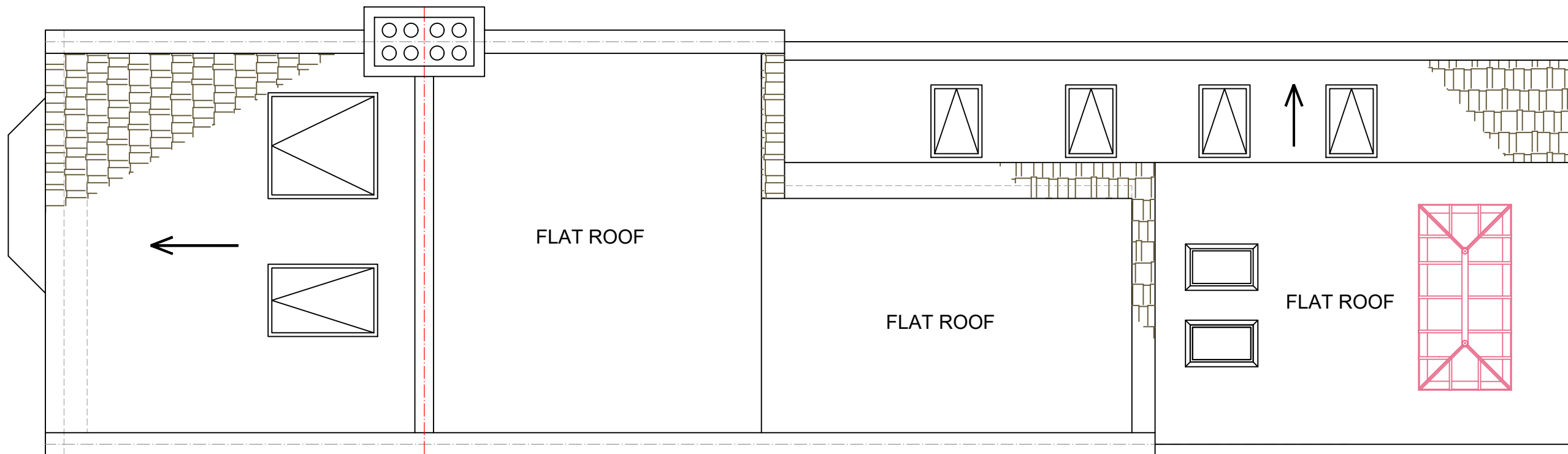
PROPOSED ROOF PLAN SCALE 1:50
